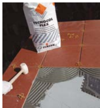
Gluing of the tiles with TECNOCOL FLEX
