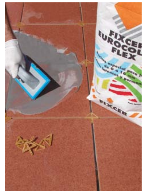
Filling the joints with EUROCOLOR FLEX
