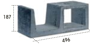
Ref. RS 902 OPEN BUILT-IN STEPS
