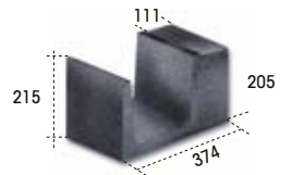
Ref. RS 913 INSIDE CORNER
